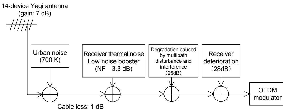
Fig. A3.2-7: Example of Distribution of the Equivalent C/N Ratio for the Reception Model
