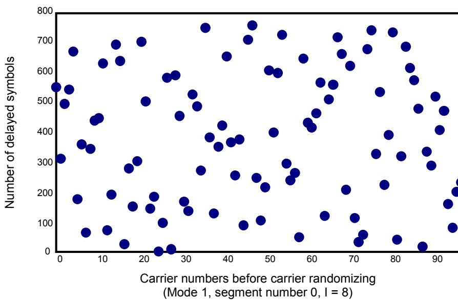
Fig. 3-28 (b): Example of Carrier Arrangement after Time Interleaving and Carrier Randomizing
