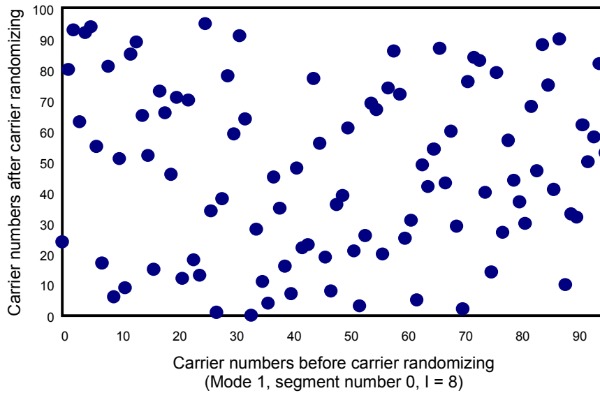
Fig. 3-28 (a): Example of Carrier Arrangement before and after Carrier Randomizing
