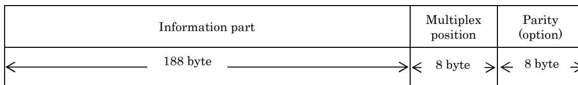
Fig. 5-10: Multiplex position on dummy byte
