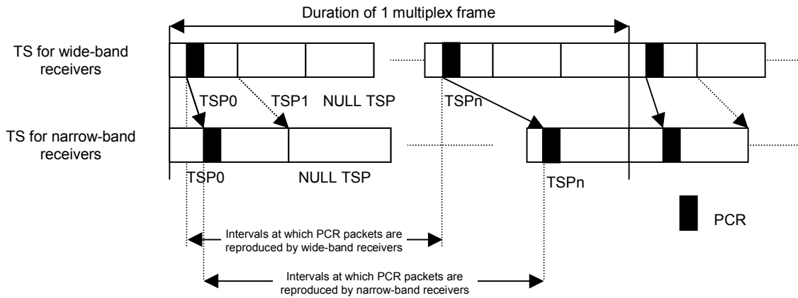
Fig. 3-2: TSs Reproduced by Wide- and Narrow-Band Receivers (No Limitations on PCR Transmission)
