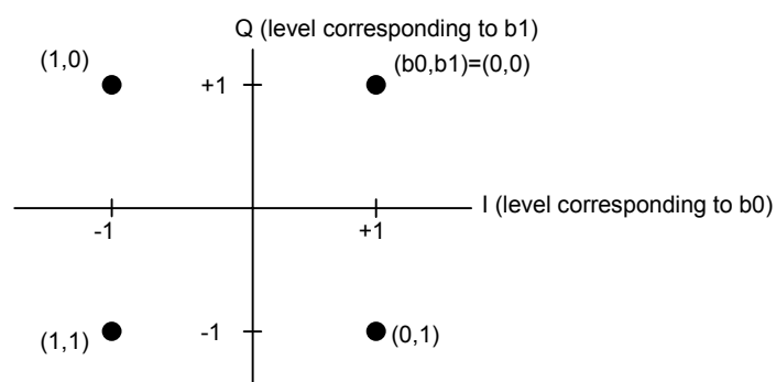
Fig. 3-15: QPSK Constellation
