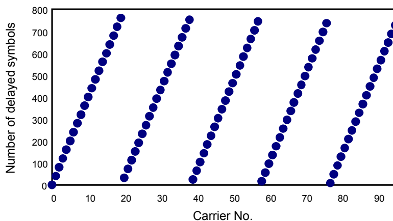
Fig. 3-24: Arrangement of Carriers Following Time Interleaving (Mode 1, l=8)
