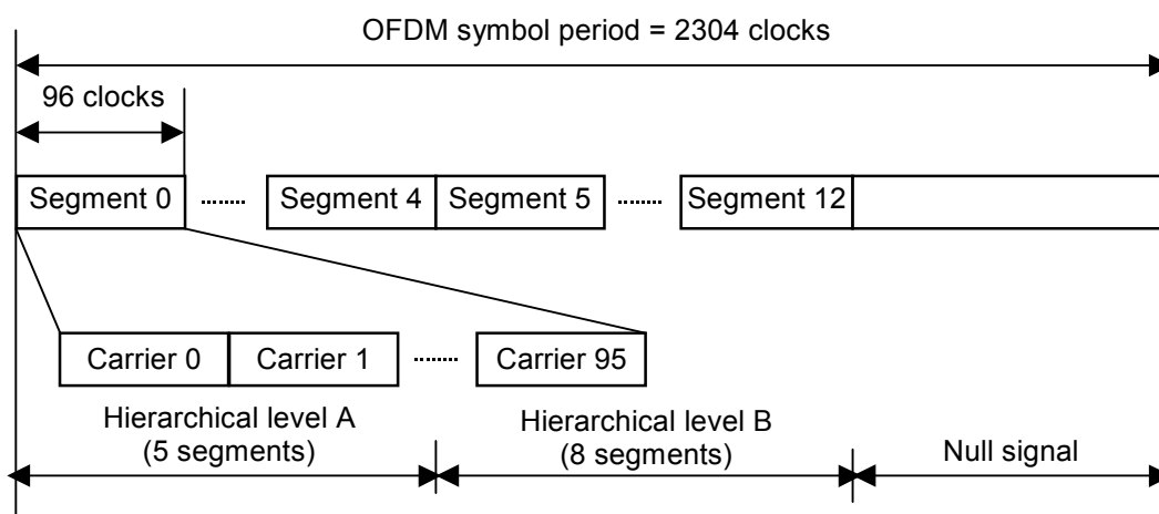
Fig. 3-5: Time Arrangement for Input Signals to Hierarchical Layers
